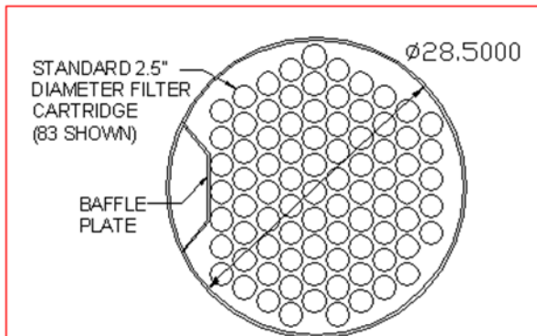
EXISTING SUMP PLATE LAYOUT WITH STANDARD CARTRIDGES
