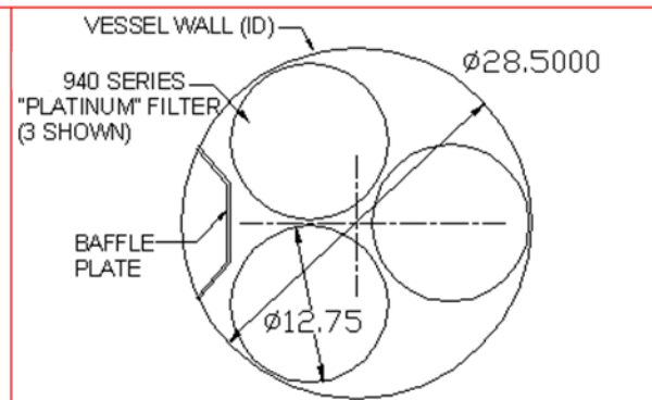
MODIFIED SUMP PLATE LAYOUT WITH "PLATINUM" PLACEMENT
